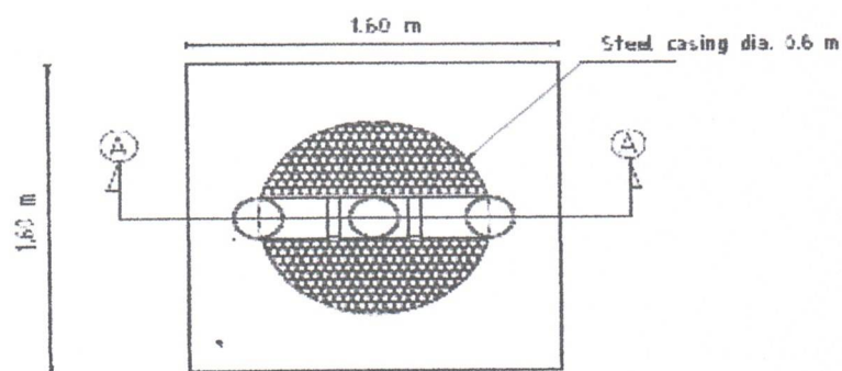
Detail 1 (Passive Vertical Vent Pipe)
